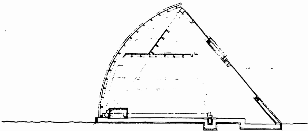
lateral section-winter
