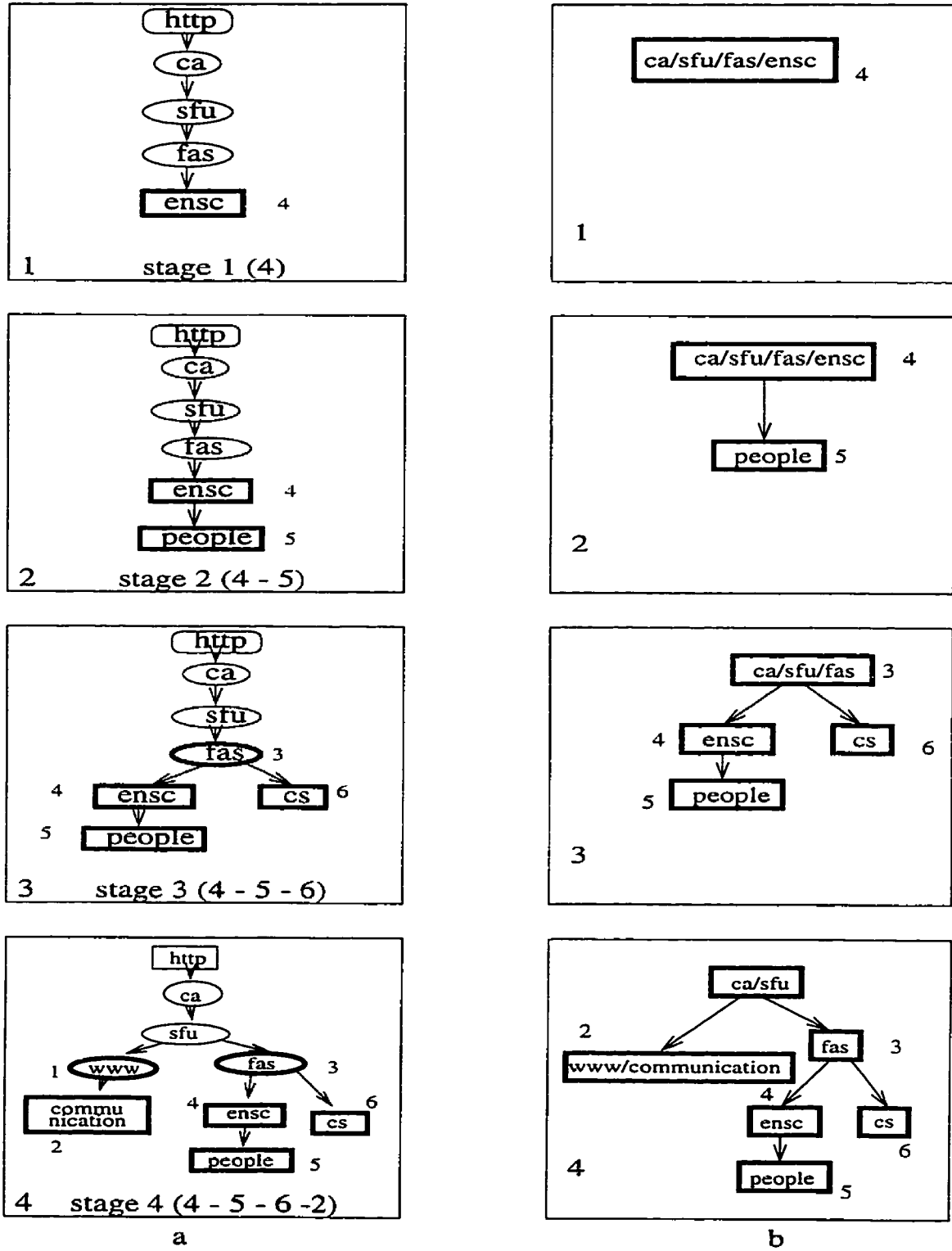
Figure 4.2: Comparison of the Internal URL-Tree and the External URL-tree
