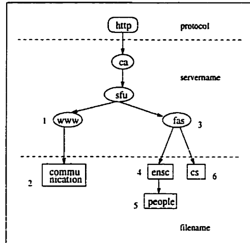
Figure 4.1: The Complete URL Tree
