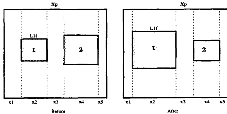
Figure 4.4: Zoom node 1 to the exact size and node 2 is resizable
