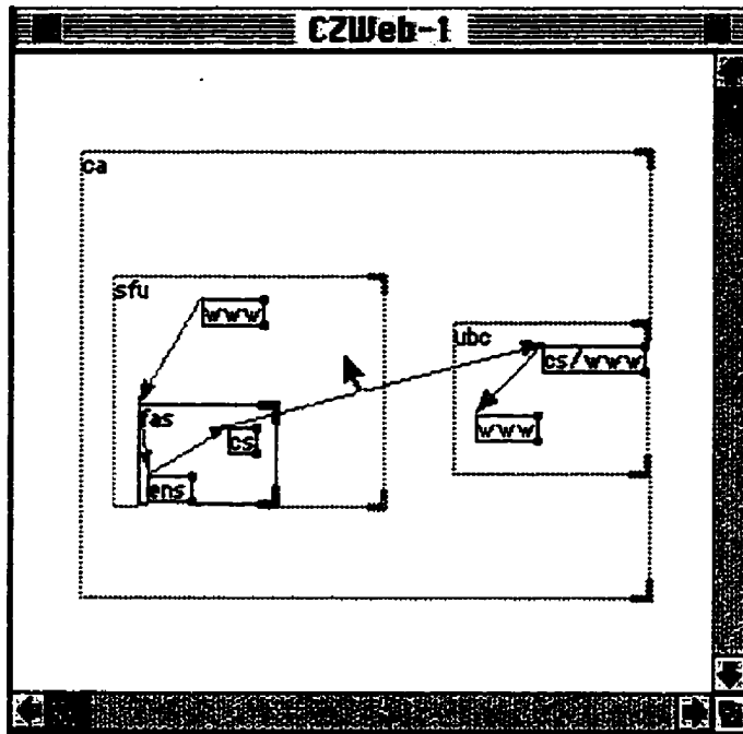
Figure 3.3: A Typical Overview of URL-tree Structure
