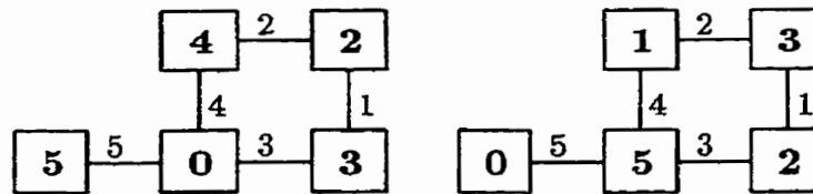
Figure 1.1 - A graceful labelling of a graph (left), with arithmetic complement (right).
