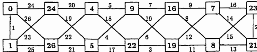
Figure 4.7: Graceful labelling of girder graph G_6 .
