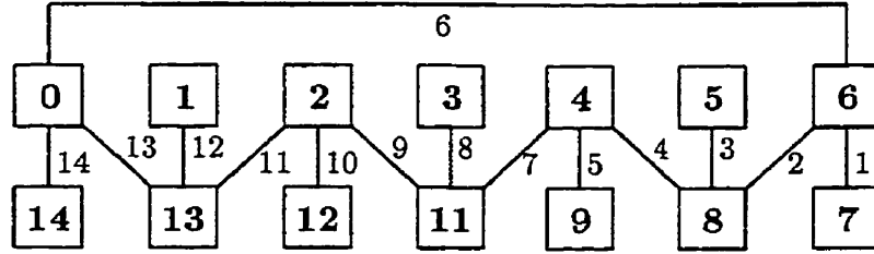
Figure 2.8: The crown graph CR_7
