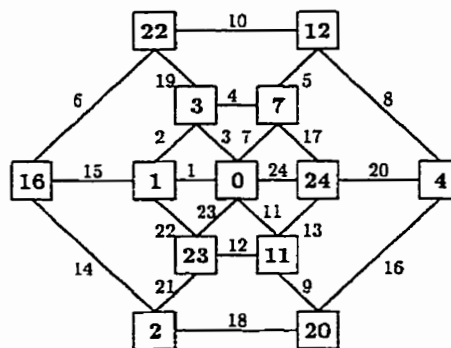
Figure 4.11: The wheel graph W(6,2) .
