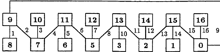
Figure 2.9: The crown graph CR_8 .
