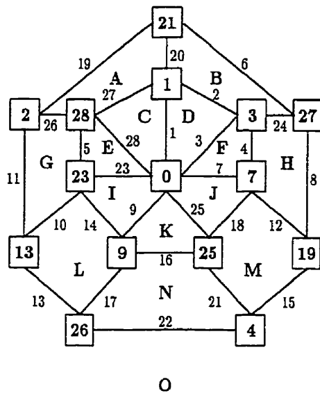
Figure 4.2: An example of a planar, graceful graph (left - the wheel graph W(7,2) ), which induces a conservative labelling of its dual graph (right). The left graph is a high-diameter wheel graph, which are defined in section 4.4.
