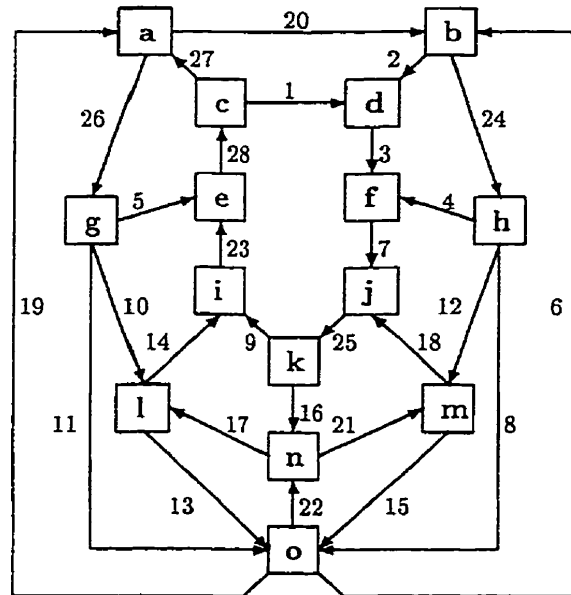
Figure 4.2: An example of a planar, graceful graph (left - the wheel graph W(7,2) ), which induces a conservative labelling of its dual graph (right). The left graph is a high-diameter wheel graph, which are defined in section 4.4.
