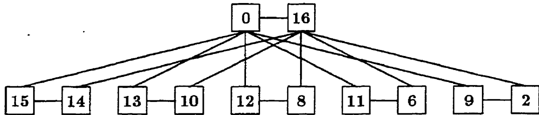
Figure 2.14: The book K_{1,5} \times P_2 , with 5 pages
