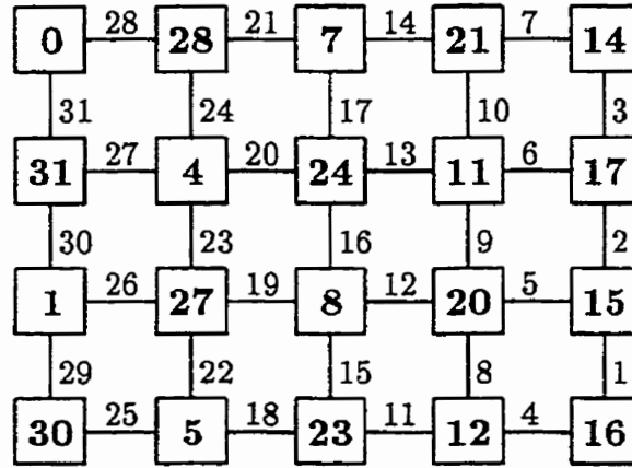
Figure 2.10: Graceful labelling of P_5 \times P_4 .
