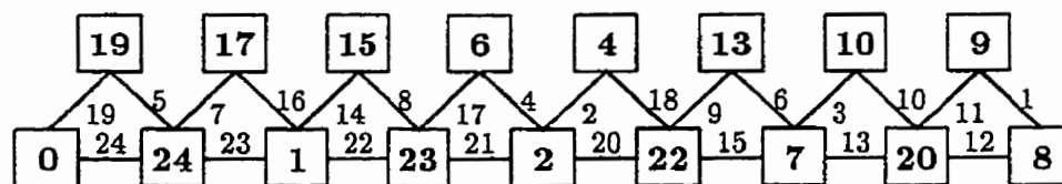
Figure 2.2: The triangular snake T_8 with graceful labelling.
