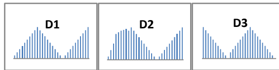
Figure 11: Visually Examining Distribution Similarity
