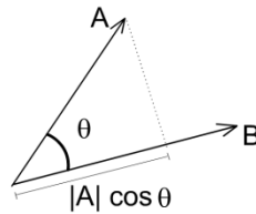
Figure 12: Geometric Representation of Two Dimensional Vectors
