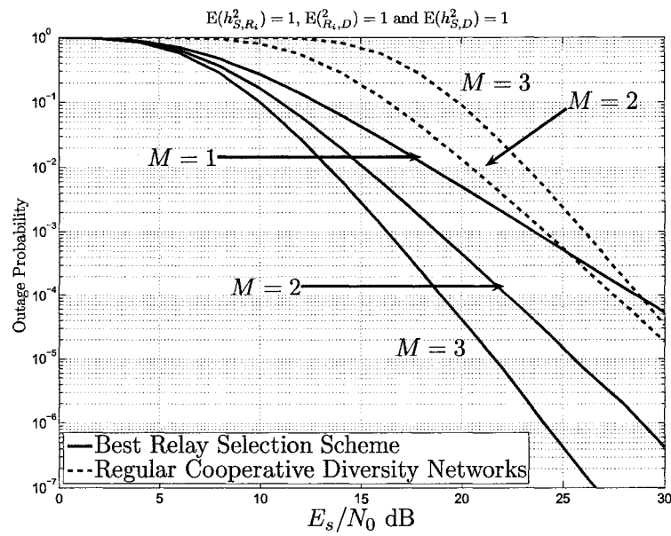
Figure 4.9: Outage probability comparison between the regular cooperative diversity with the best-relay selection cooperative diversity over Rayleigh fading channels. Note that for M = 1 regular and path-selection schemes have the same outage probability.
