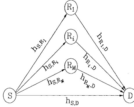
Figure 2.1: Illustration of a multi branch cooperative diversity network.
