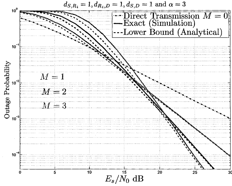
Figure 2.4: Outage Probability for amplify-and-forward wireless cooperative diversity networks for m_{S,D} = 1 , m_{S,R_i} = 0.5 , and m_{R_i,D} = 1 .
