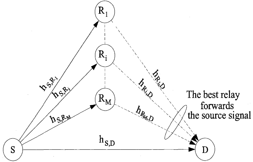
Figure 4.1: Illustration of a multi branch cooperative diversity network.
