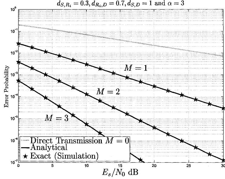
Figure 2.3: Error Probability for decode-and-forward wireless cooperative diversity networks for m_{S,D} = 0.5 , m_{S,R_i} = 0.5 , and m_{R_i,D} = 1 .
