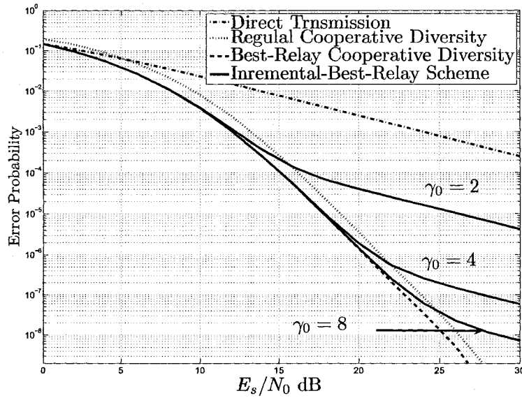
Figure 6.2: Error performance for the decode-and-forward incremental-best-relay selection scheme over Rayleigh fading channels.
