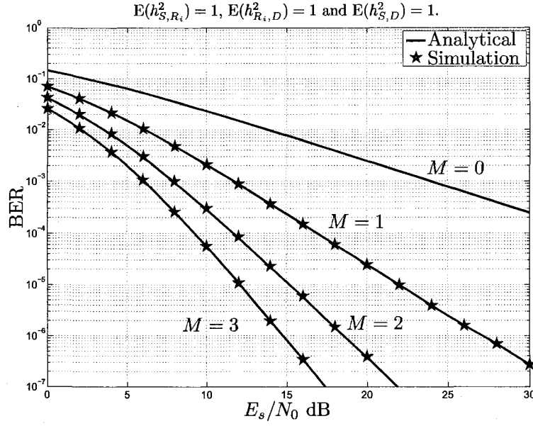
Figure 4.6: Error performance for the best- relay selection scheme over Rayleigh fading channels.
