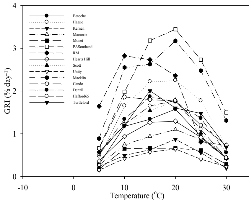
Fig. 5.3 Germination rate index (GRI) of 15 F. hallii populations in six different temperature regimes from 5-30°C.
