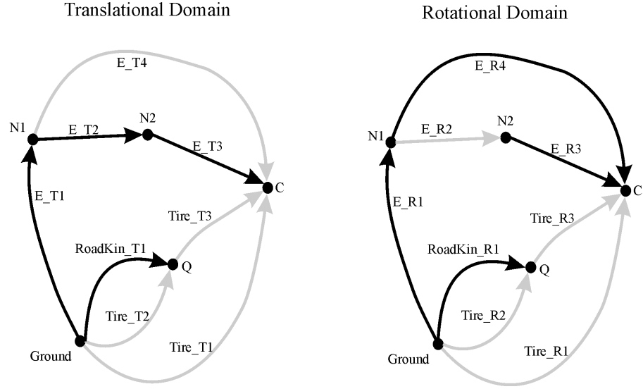
Figure 4.4: A Linear Graph with Tire Component
