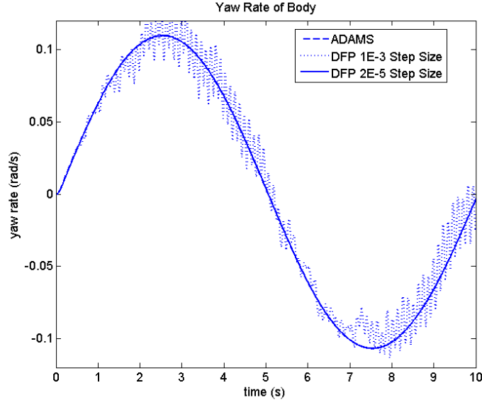
Figure 5.12: Yaw Rate Response of Generic 4-Wheeled Vehicle for Sine Steer Maneuver – Simulation Code Generated with Tire Edges T1 and R1 in Tree
